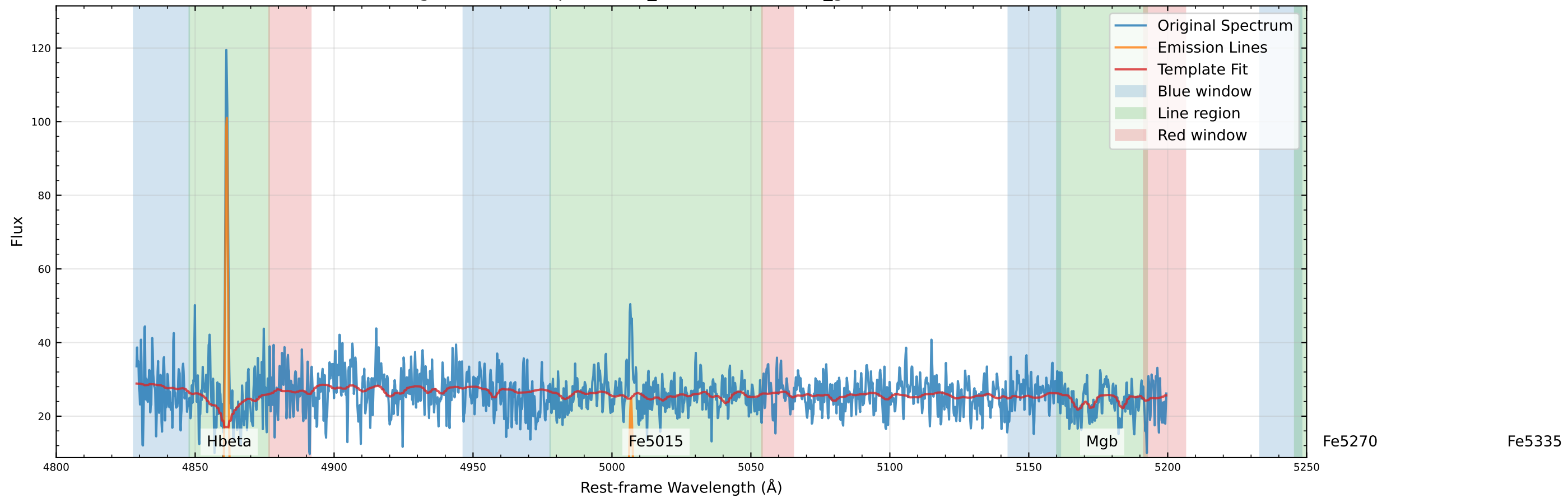
Original Data Comparison ( v_{\text{star}}=-15.5 km/s, v_{\text{gas}}=-0.0 km/s)
