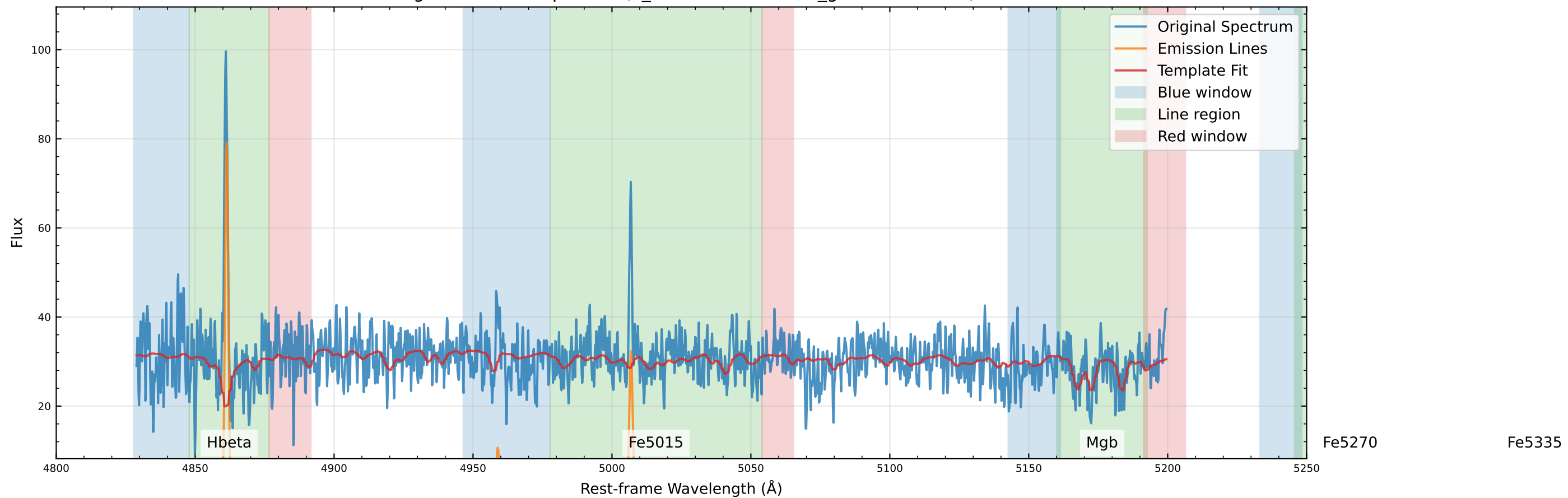
Original Data Comparison (v_star=-34.1 km/s, v_gas=-16.1 km/s)
