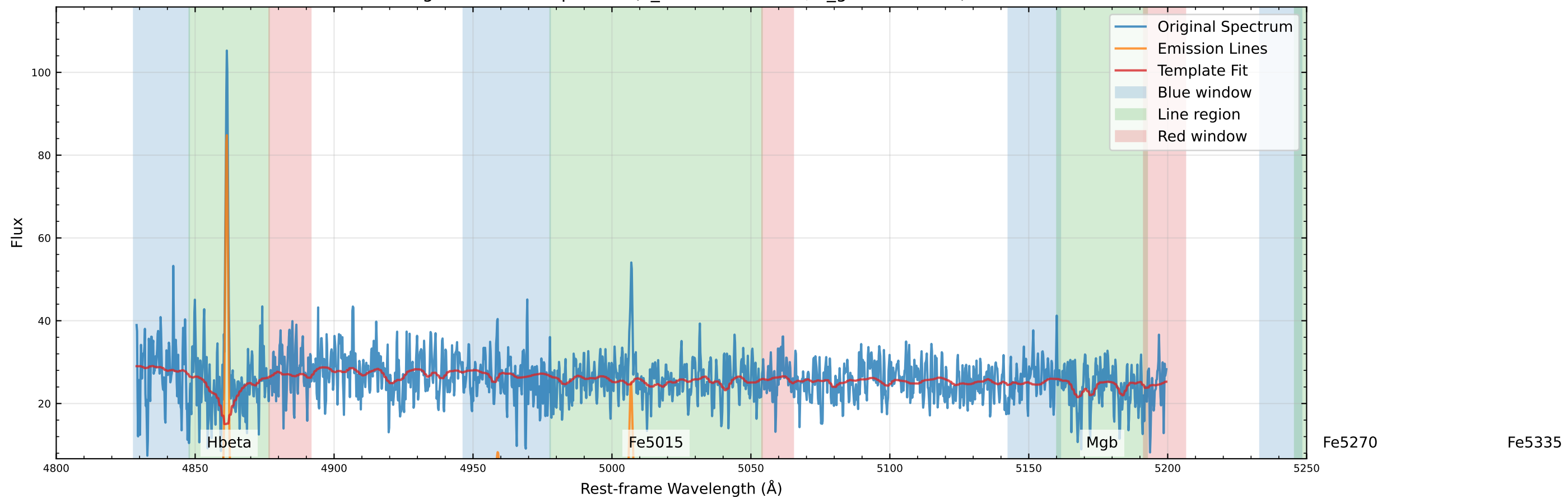
Original Data Comparison (v_star=-14.1 km/s, v_gas=2.2 km/s)
