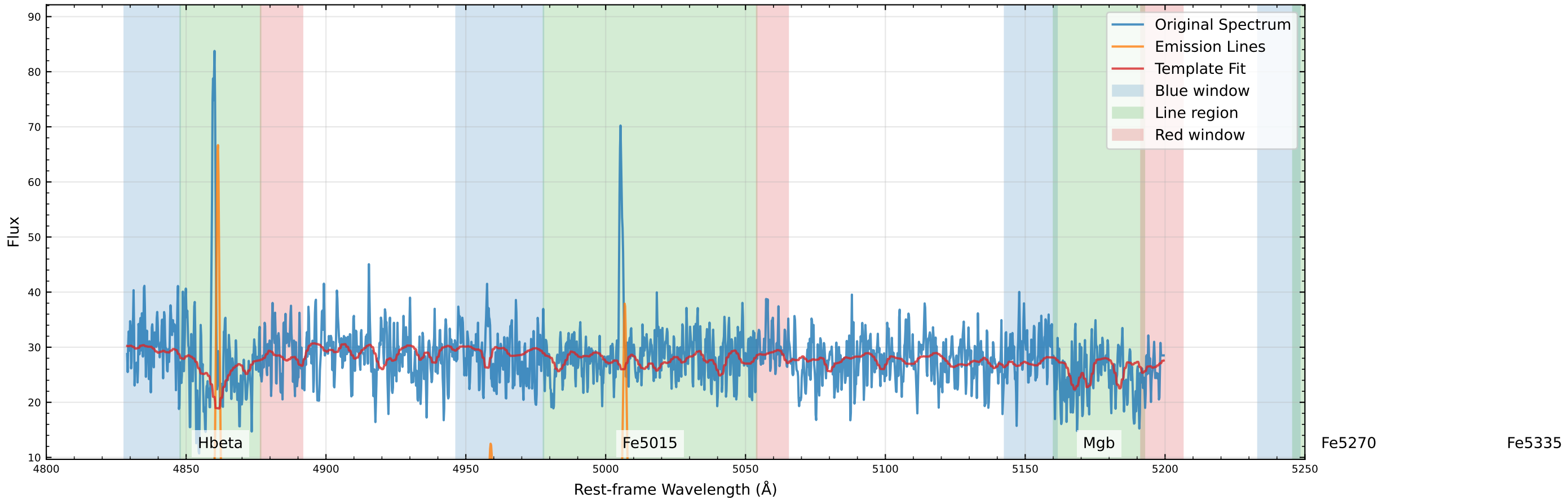
Original Data Comparison (v_star=-118.2 km/s, v_gas=-87.6 km/s)
