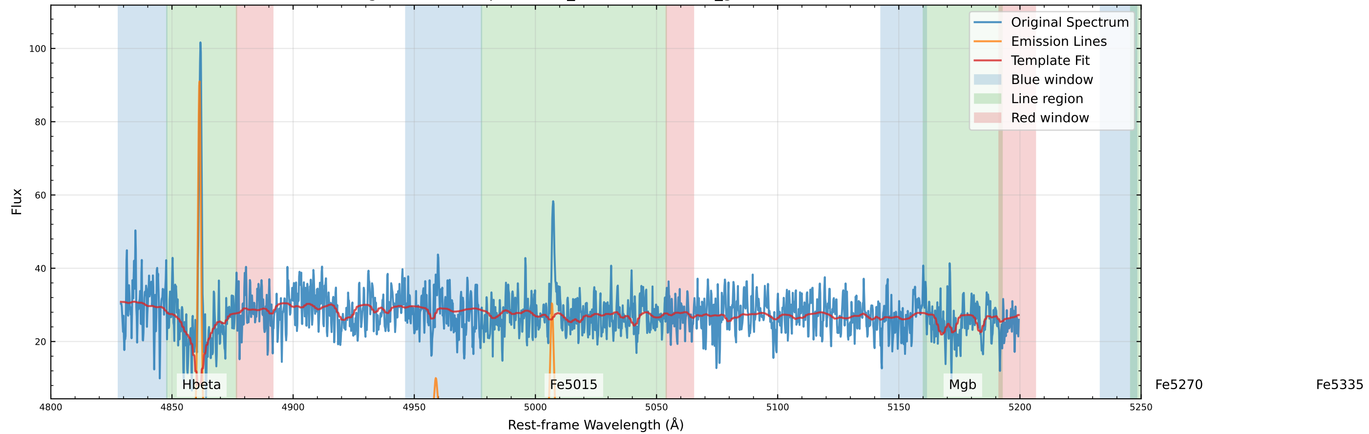
Original Data Comparison (v_star=43.8 km/s, v_gas=22.5 km/s)
