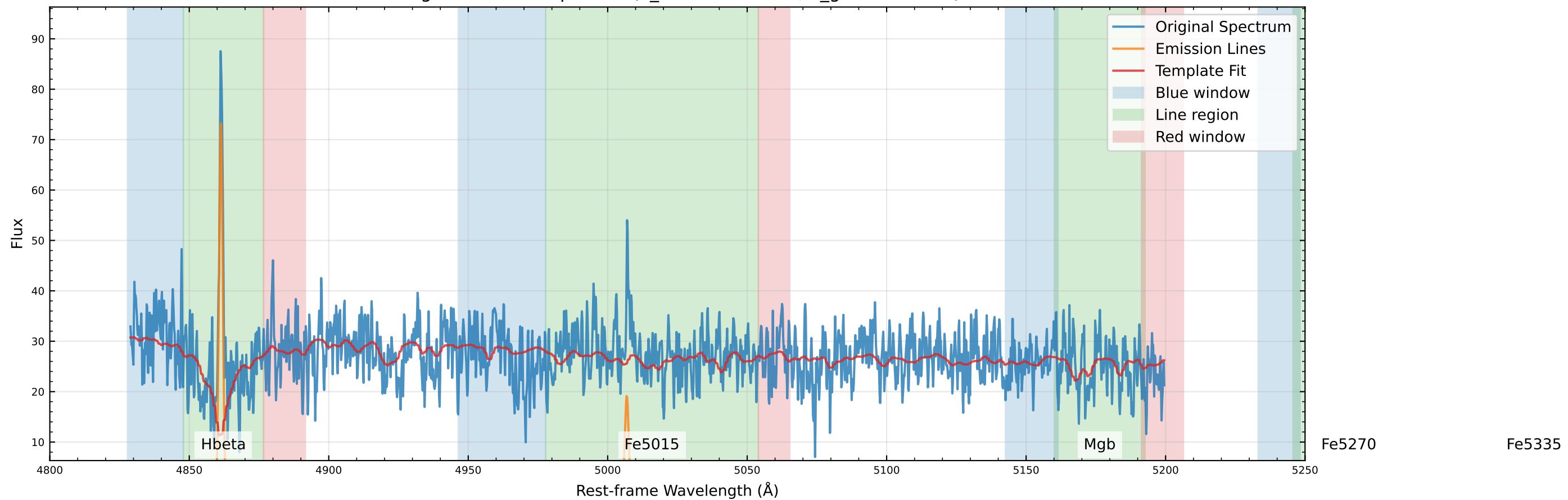
Original Data Comparison (v_star=11.9 km/s, v_gas=5.9 km/s)
