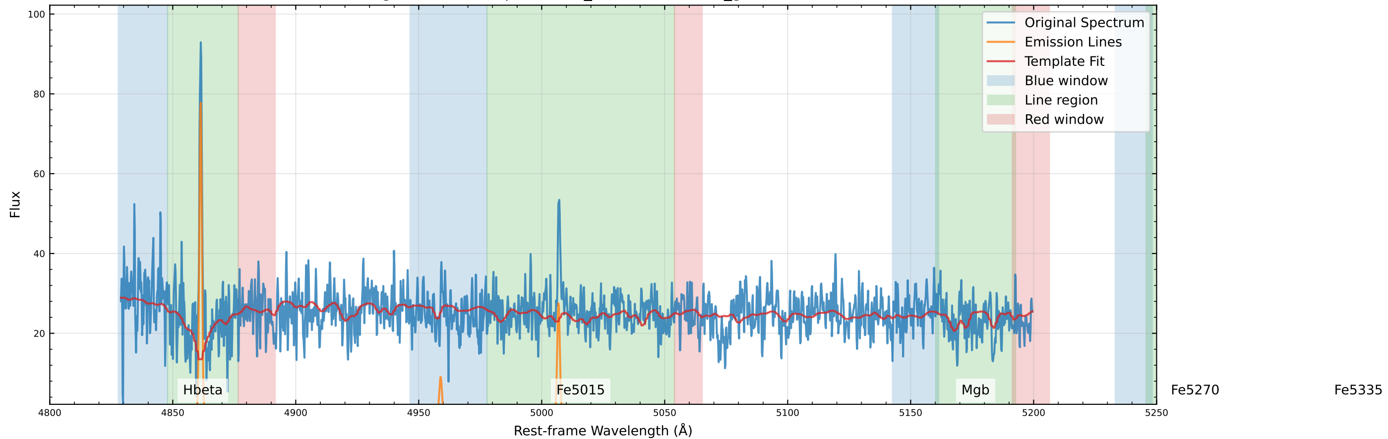
Original Data Comparison (v_star=1.3 km/s, v_gas=3.2 km/s)
