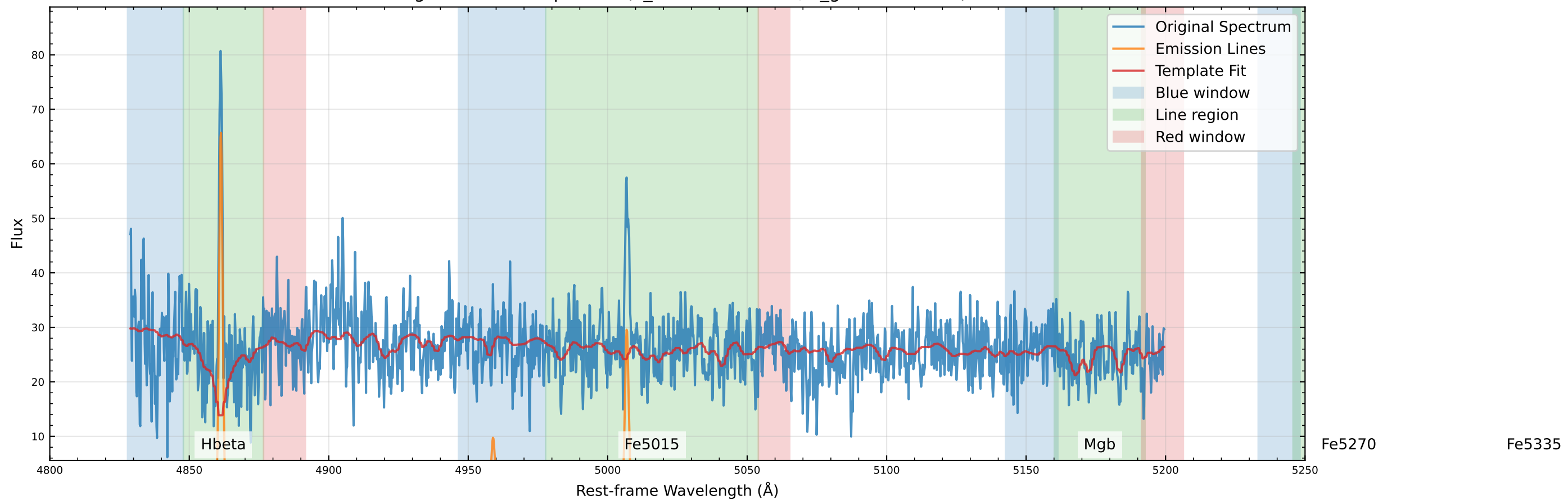
Original Data Comparison (v_star=-15.0 km/s, v_gas=-3.3 km/s)
