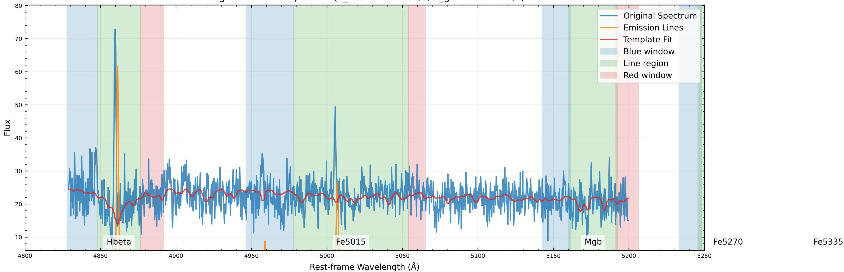
Original Data Comparison (v_star=-71.8 km/s, v_gas=-99.9 km/s)
