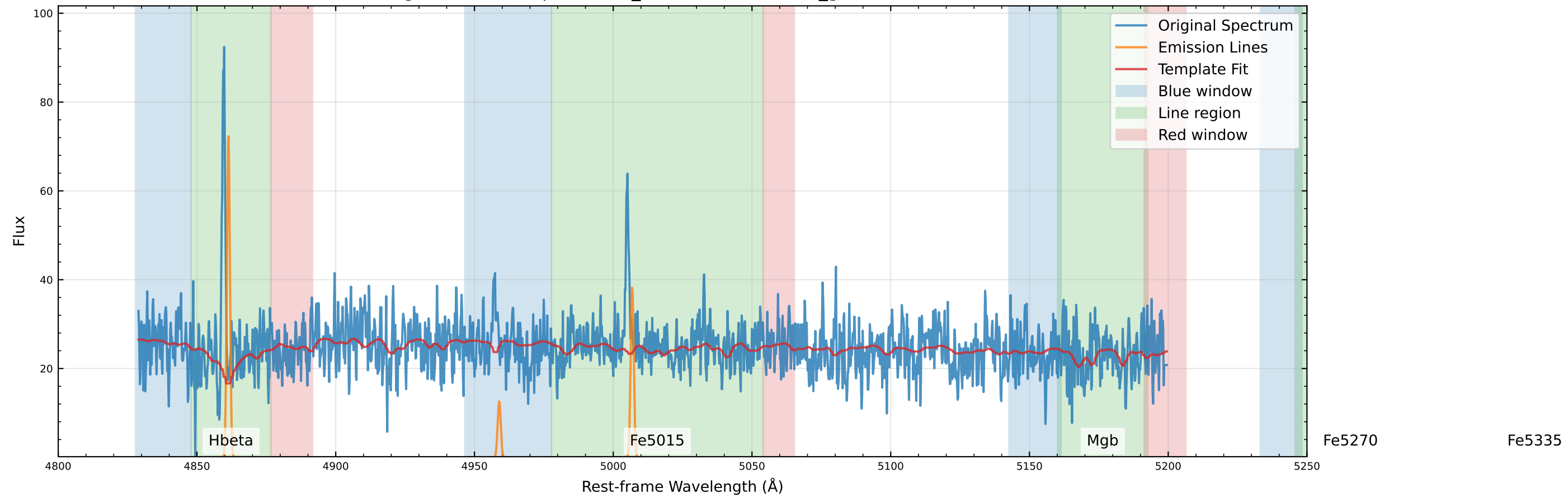
Original Data Comparison (v_star=-112.0 km/s, v_gas=-106.7 km/s)
