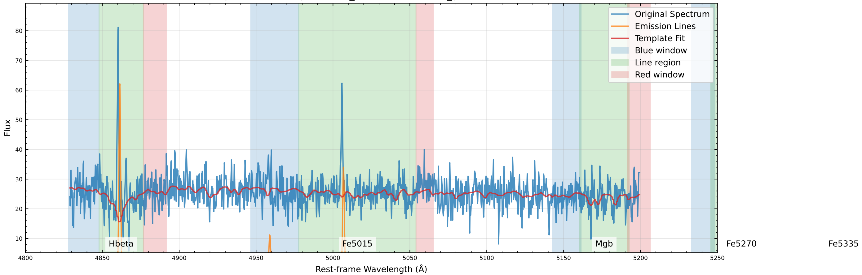
Original Data Comparison (v_star=-74.7 km/s, v_gas=-66.9 km/s)
