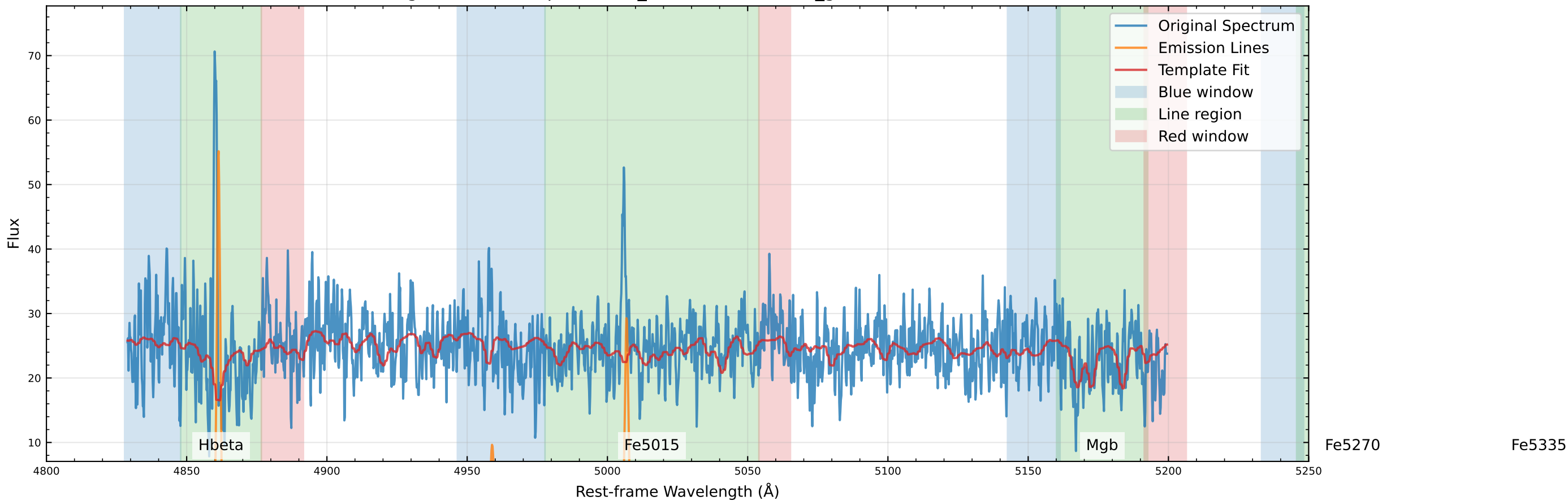
Original Data Comparison (v_star=-48.8 km/s, v_gas=-67.2 km/s)
