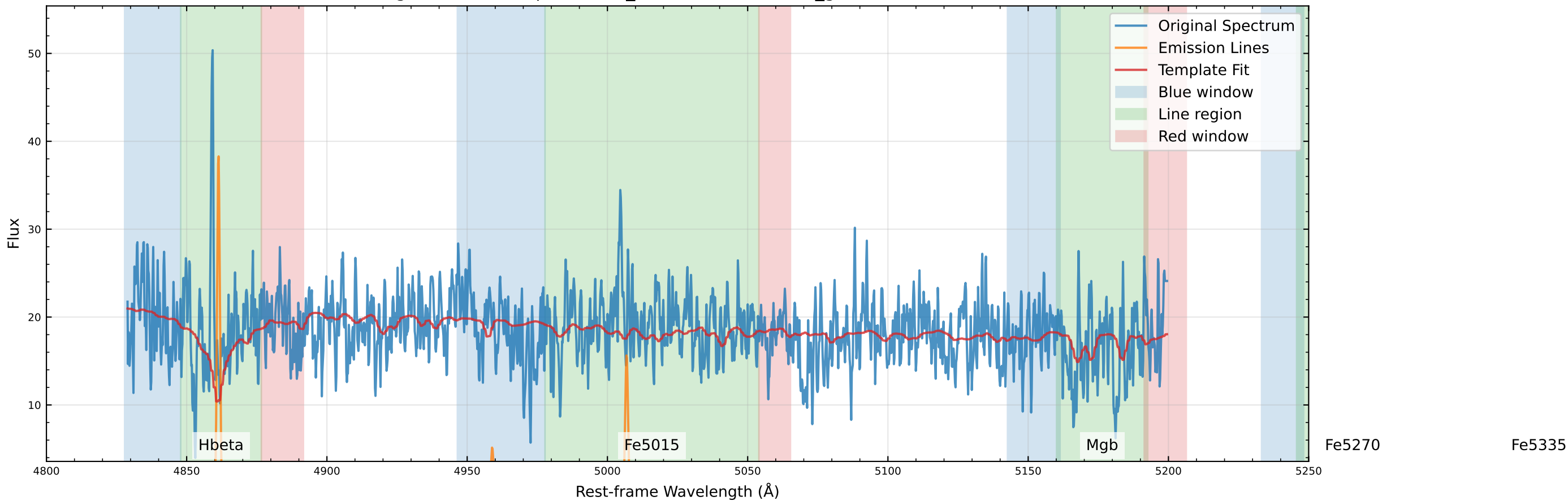
Original Data Comparison (v_star=-132.8 km/s, v_gas=-137.6 km/s)
