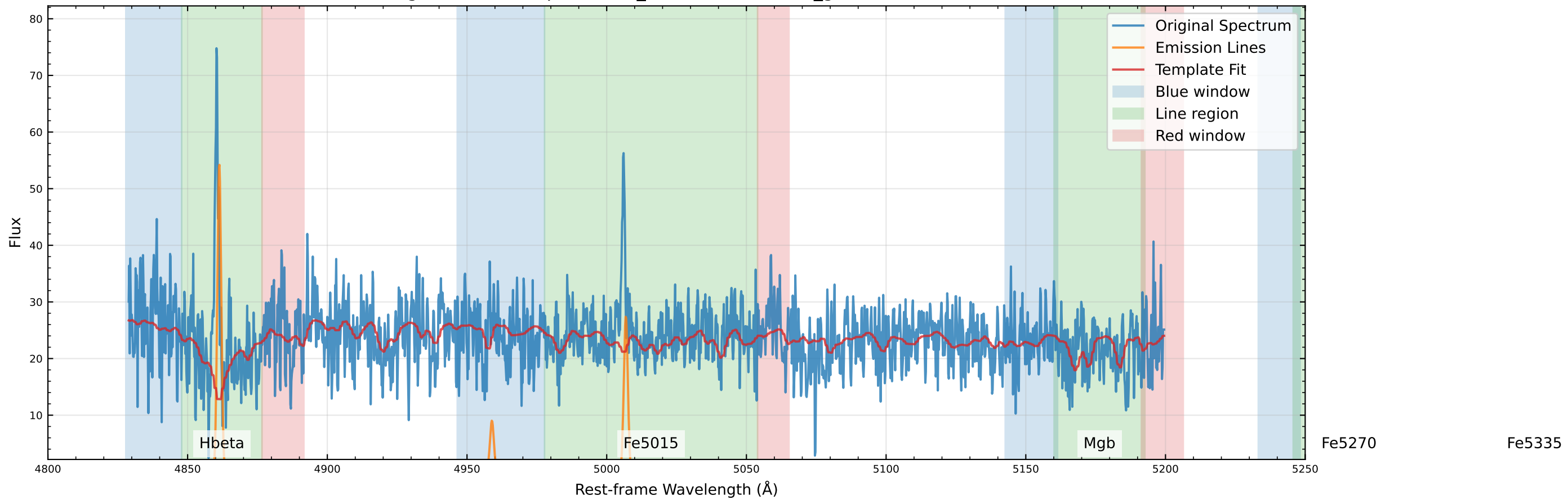
Original Data Comparison (v_star=-46.9 km/s, v_gas=-56.9 km/s)
