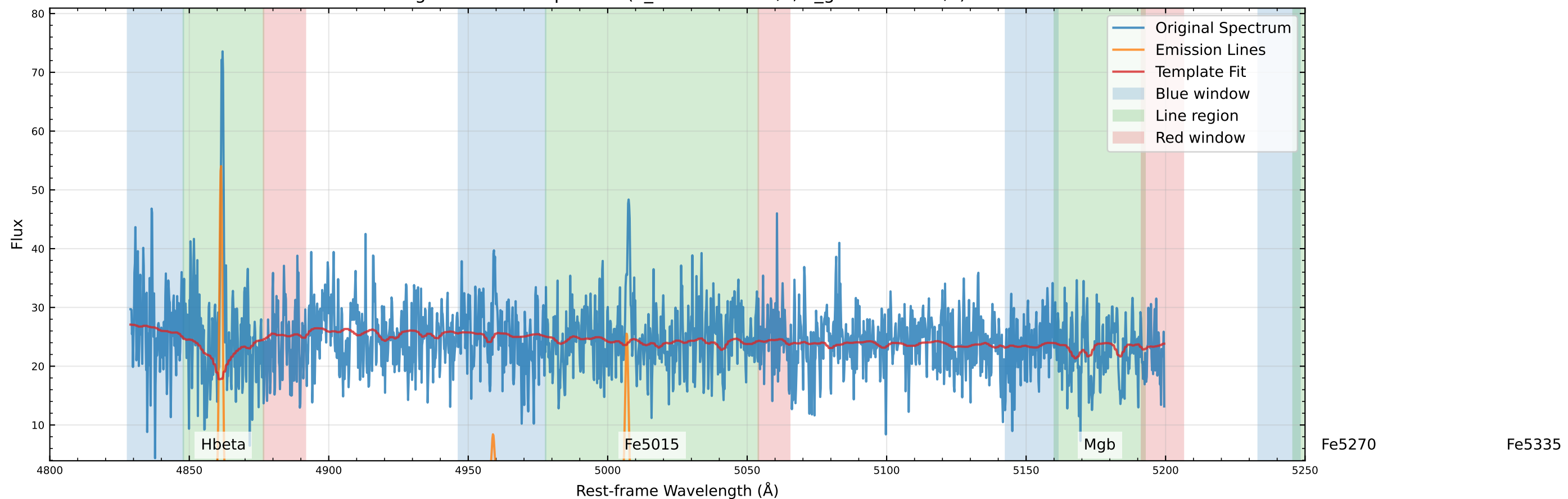
Original Data Comparison (v_star=44.2 km/s, v_gas=30.7 km/s)
