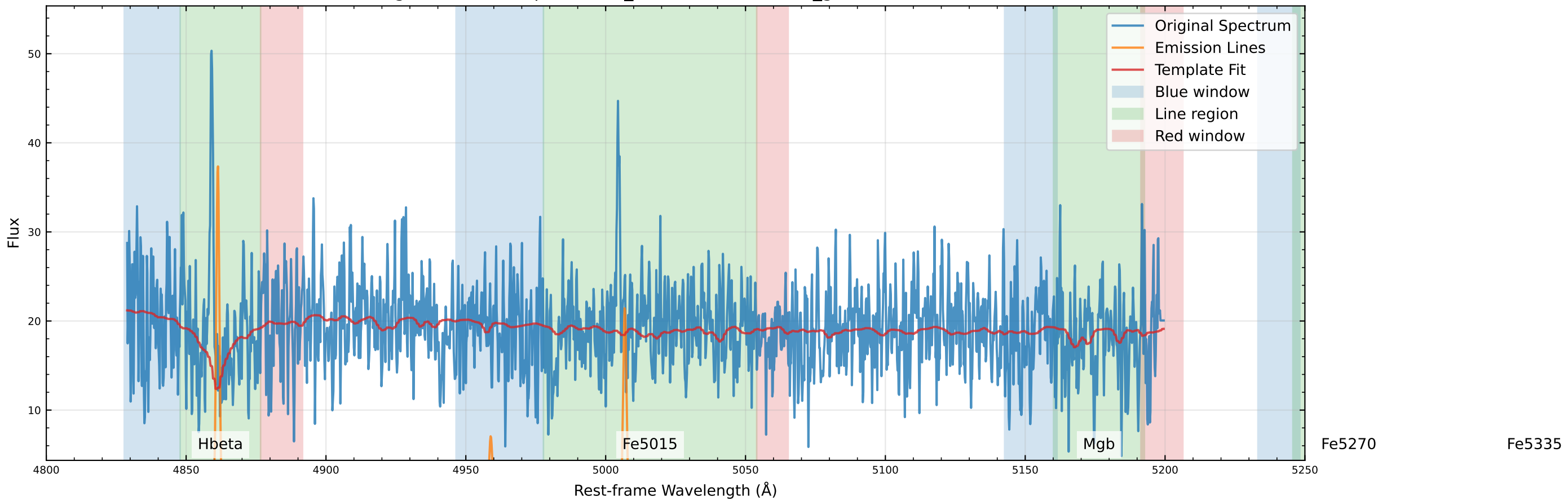
Original Data Comparison (v_star=-148.2 km/s, v_gas=-139.2 km/s)
