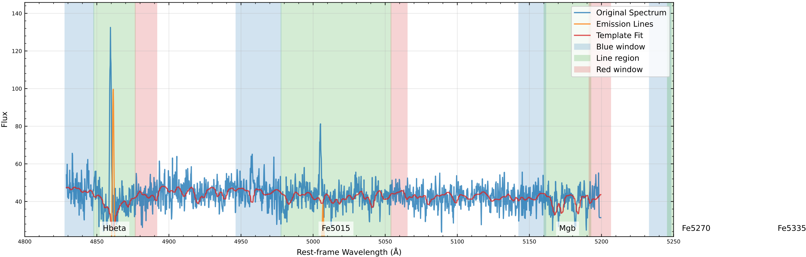
Original Data Comparison (v_star=-126.3 km/s, v_gas=-113.3 km/s)
