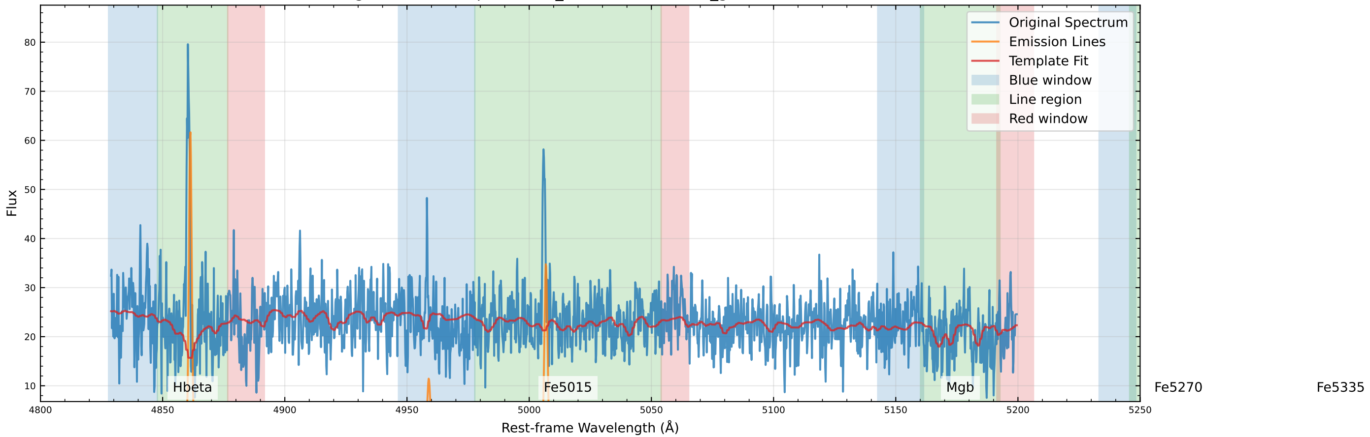
Original Data Comparison (v_star=-64.4 km/s, v_gas=-54.5 km/s)
