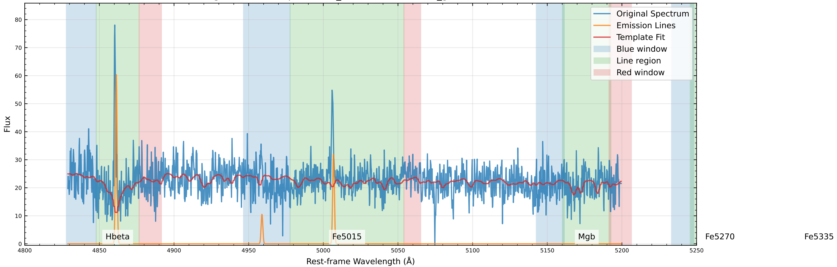
Original Data Comparison (v_star=-118.1 km/s, v_gas=-54.6 km/s)
