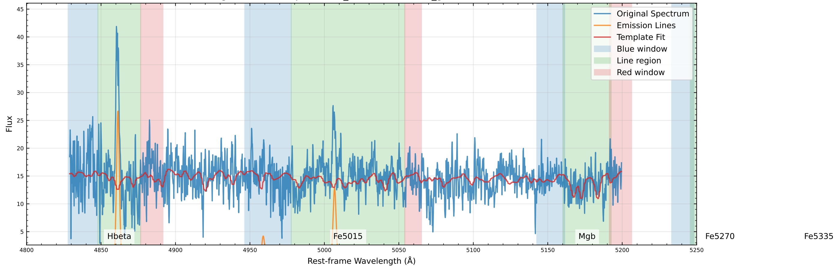
Original Data Comparison (v_star=-2.2 km/s, v_gas=-23.3 km/s)
