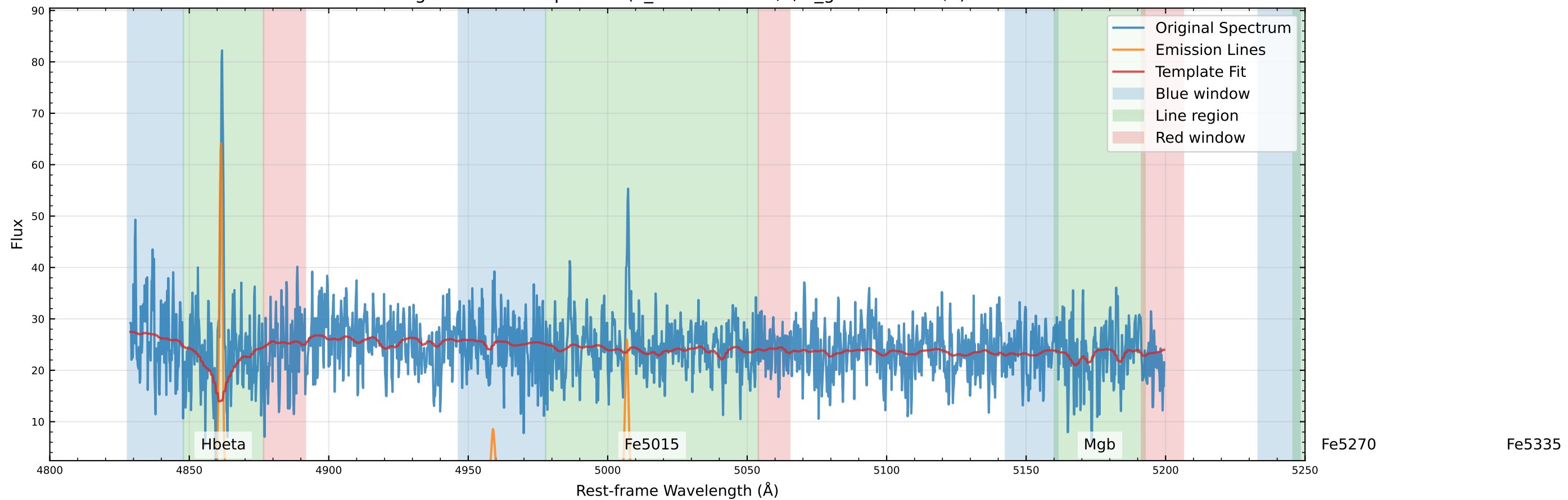
Original Data Comparison (v_star=24.5 km/s, v_gas=21.8 km/s)
