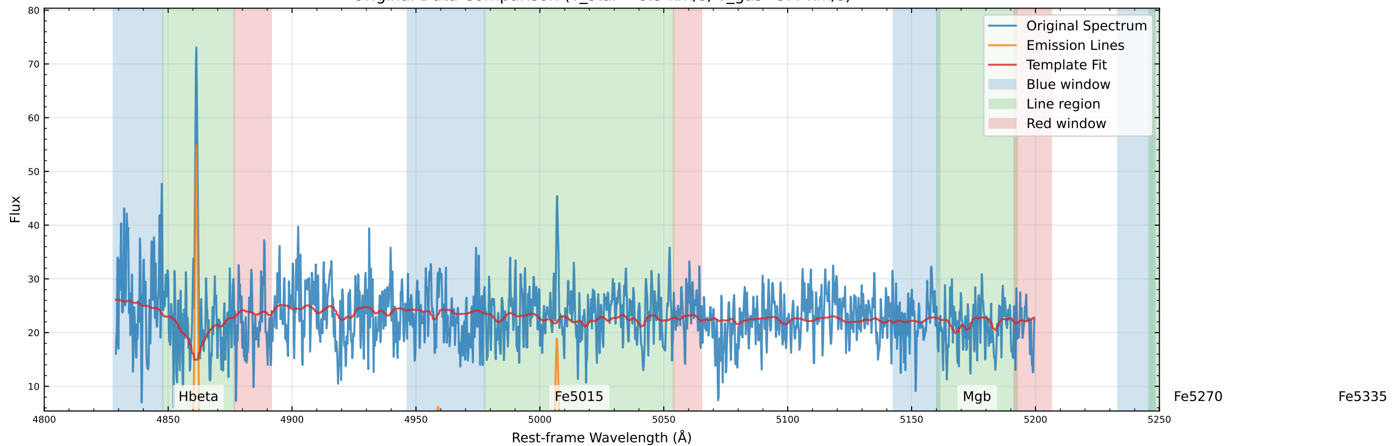
Original Data Comparison (v_star=-8.3 km/s, v_gas=3.4 km/s)
