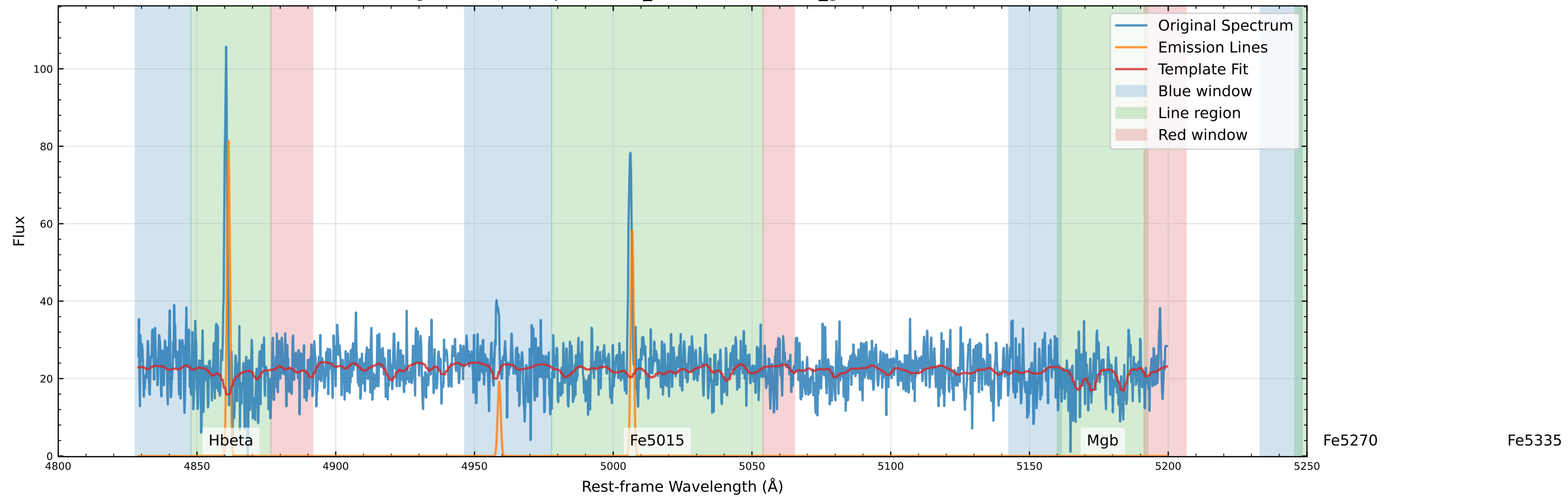
Original Data Comparison (v_star=-62.1 km/s, v_gas=-53.6 km/s)
