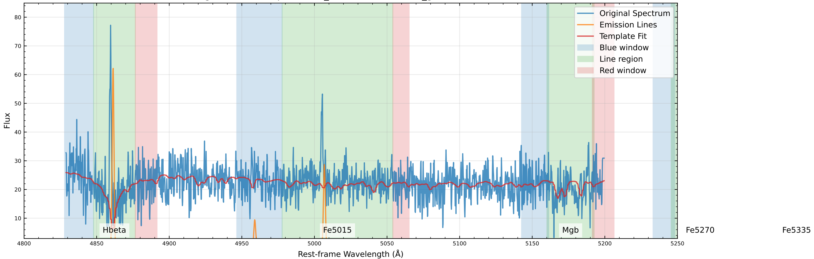
Original Data Comparison (v_star=-123.1 km/s, v_gas=-109.6 km/s)
