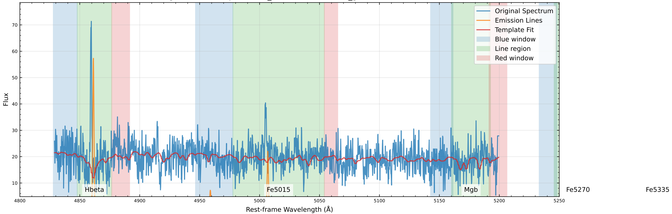
Original Data Comparison (v_star=-110.6 km/s, v_gas=-119.0 km/s)
