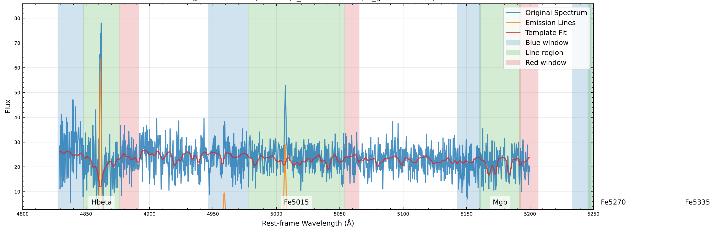
Original Data Comparison (v_star=-2.1 km/s, v_gas=7.7 km/s)
