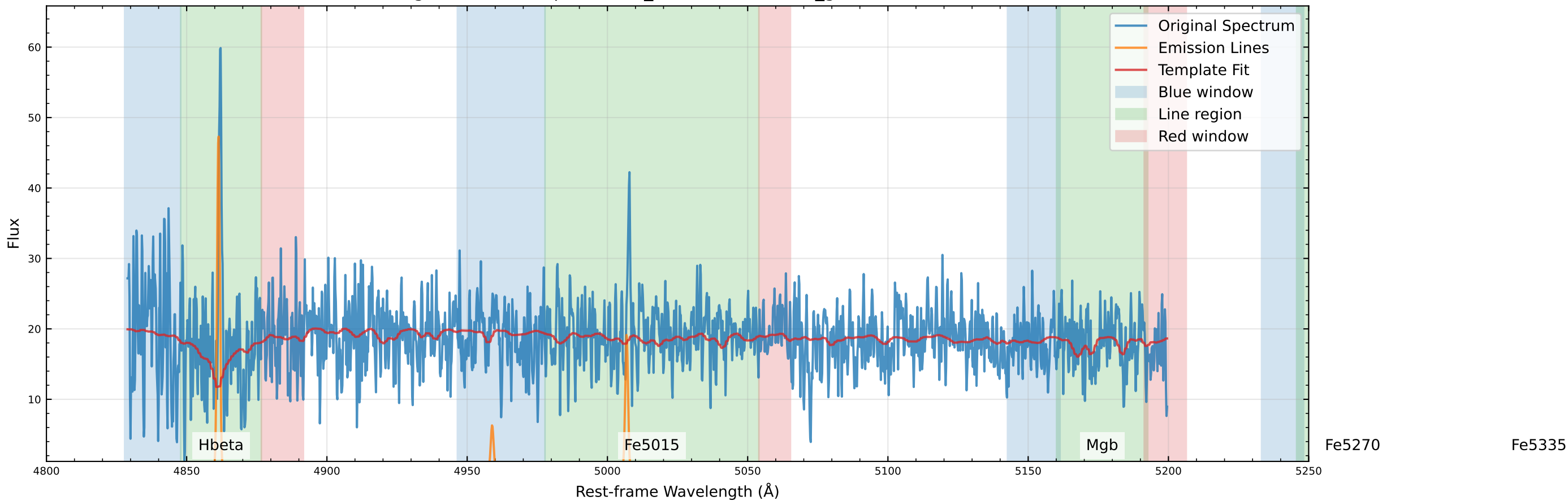
Original Data Comparison (v_star=49.7 km/s, v_gas=41.2 km/s)
