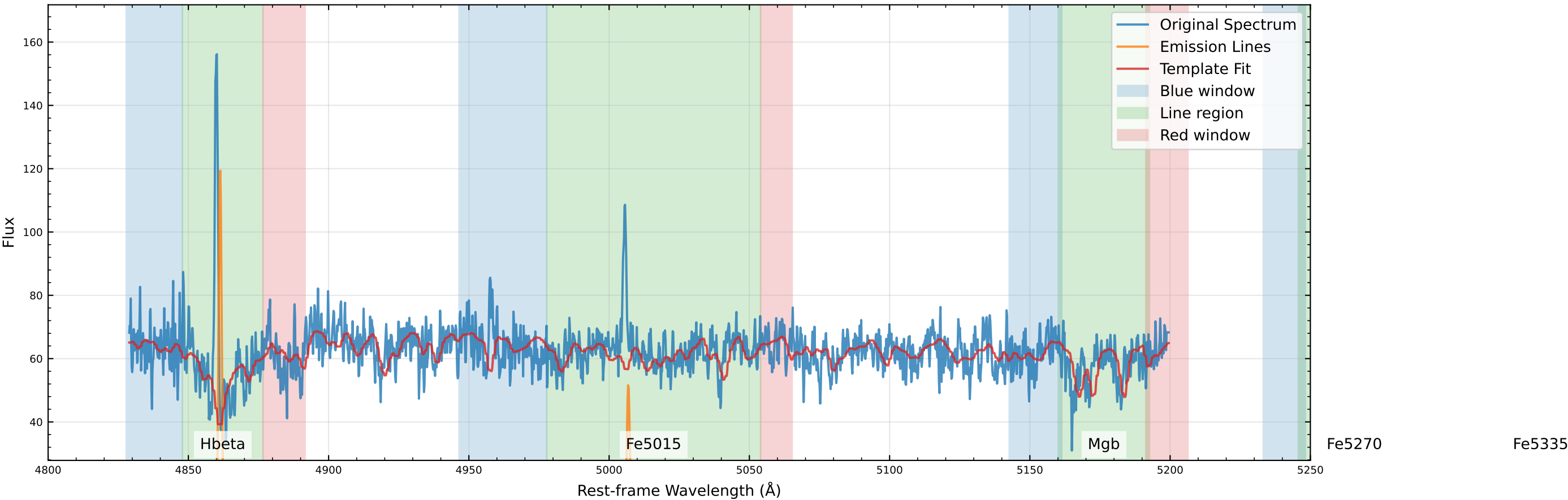
Original Data Comparison (v_star=-89.7 km/s, v_gas=-83.7 km/s)
