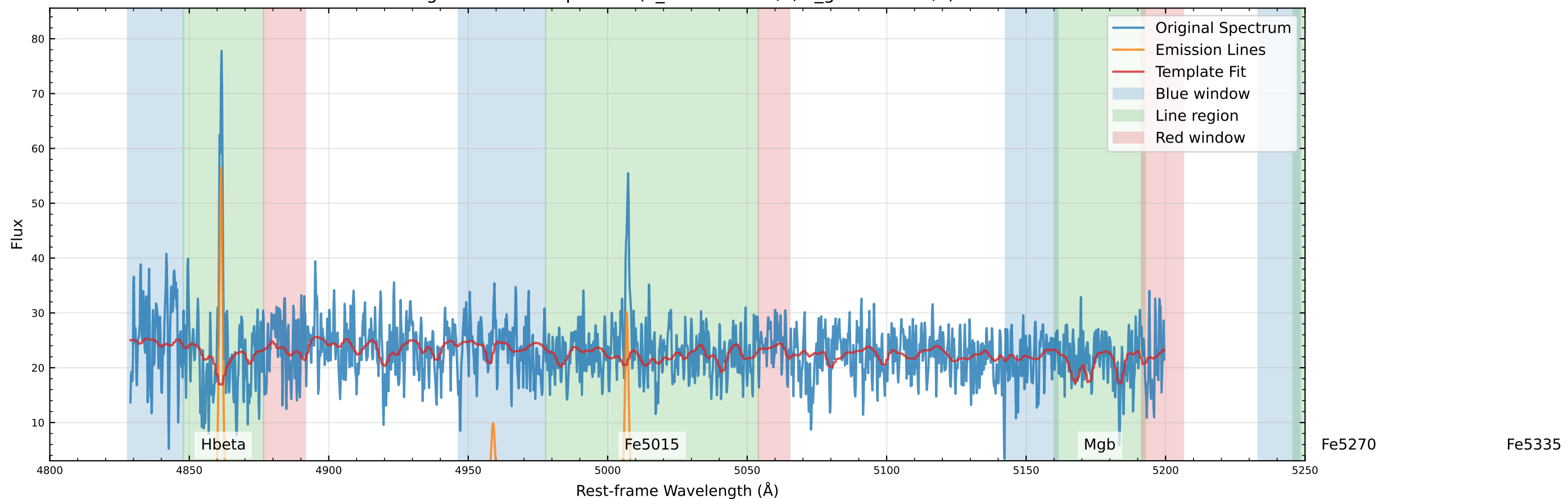
Original Data Comparison (v_star=8.5 km/s, v_gas=7.3 km/s)
