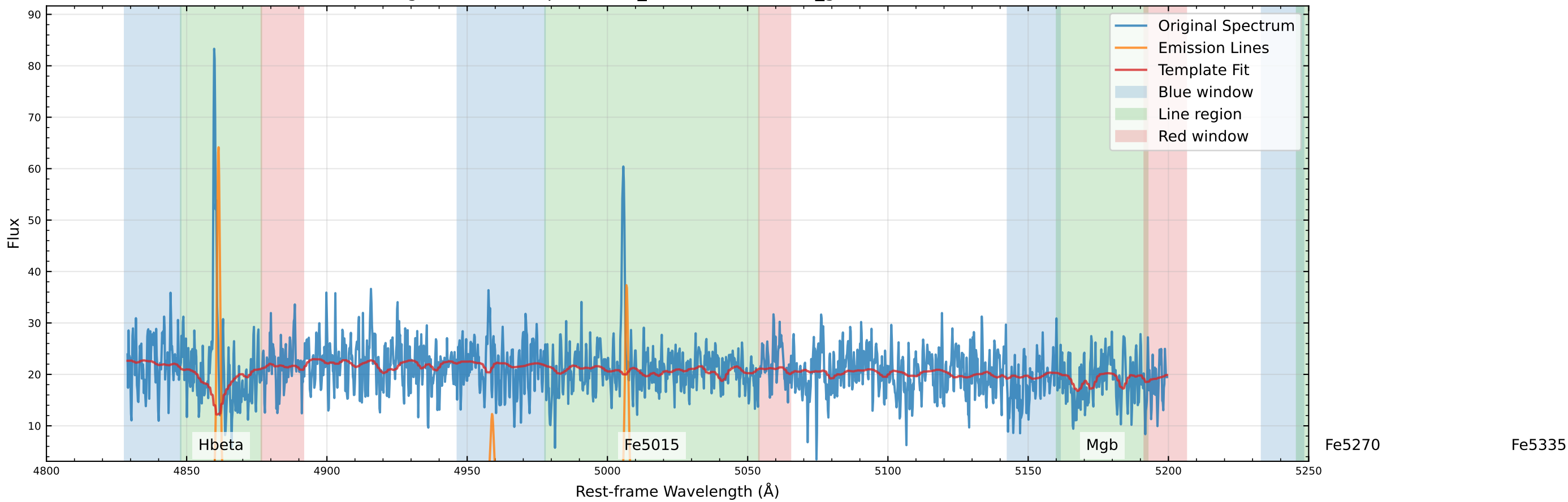
Original Data Comparison (v_star=-49.2 km/s, v_gas=-79.3 km/s)
