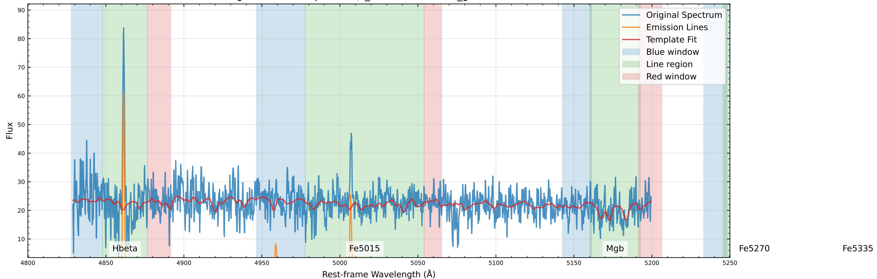
Original Data Comparison (v_star=-8.6 km/s, v_gas=3.6 km/s)
