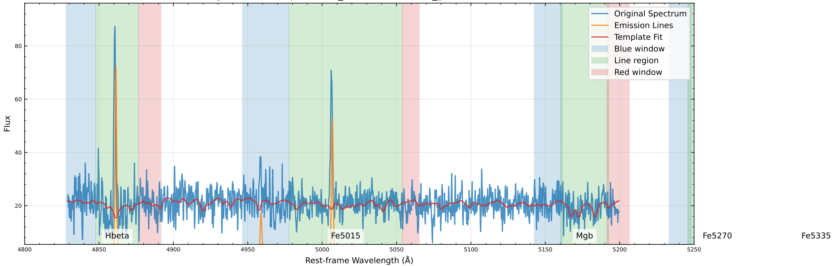
Original Data Comparison (v_star=-37.1 km/s, v_gas=-43.1 km/s)
