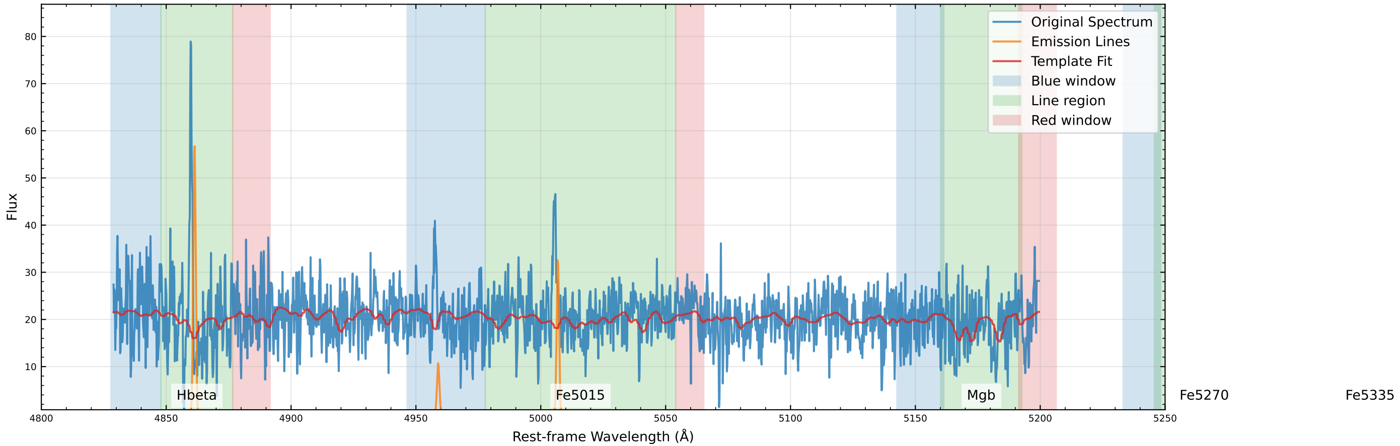
Original Data Comparison (v_star=-108.0 km/s, v_gas=-87.8 km/s)
