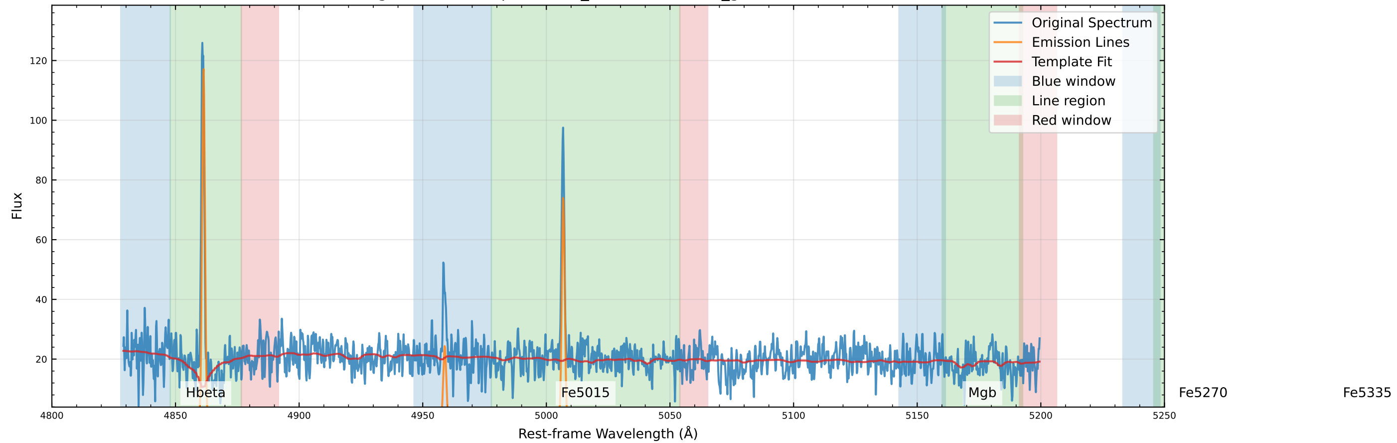
Original Data Comparison (v_star=8.4 km/s, v_gas=-15.9 km/s)
