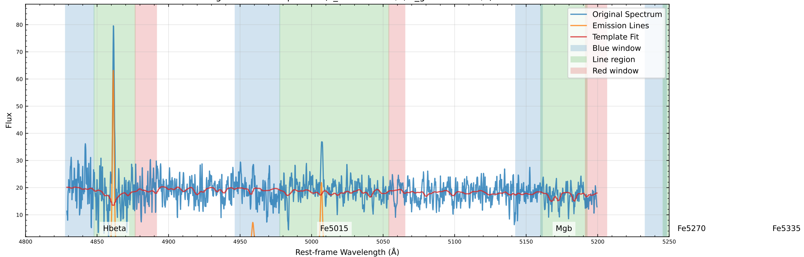
Original Data Comparison (v_star=3.8 km/s, v_gas=12.8 km/s)
