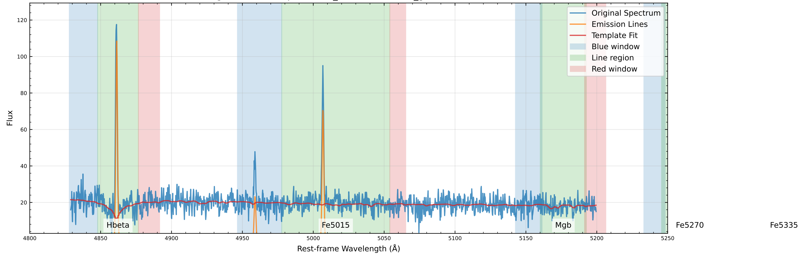
Original Data Comparison (v_star=4.9 km/s, v_gas=-12.6 km/s)
