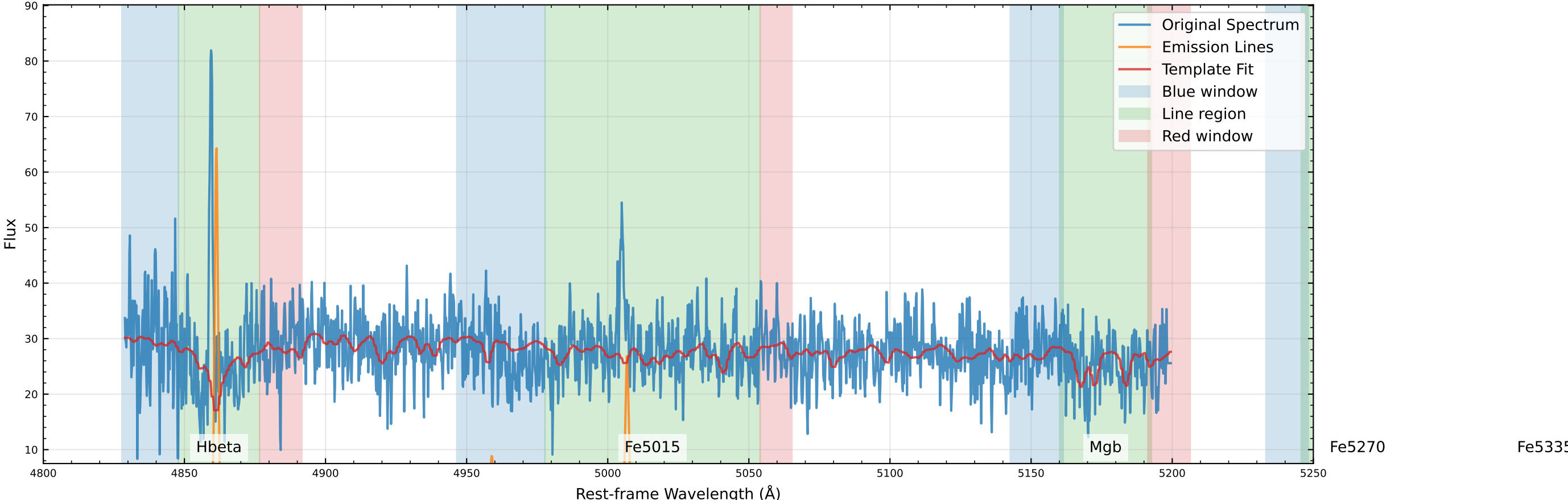
Original Data Comparison (v_star=-127.9 km/s, v_gas=-116.7 km/s)
