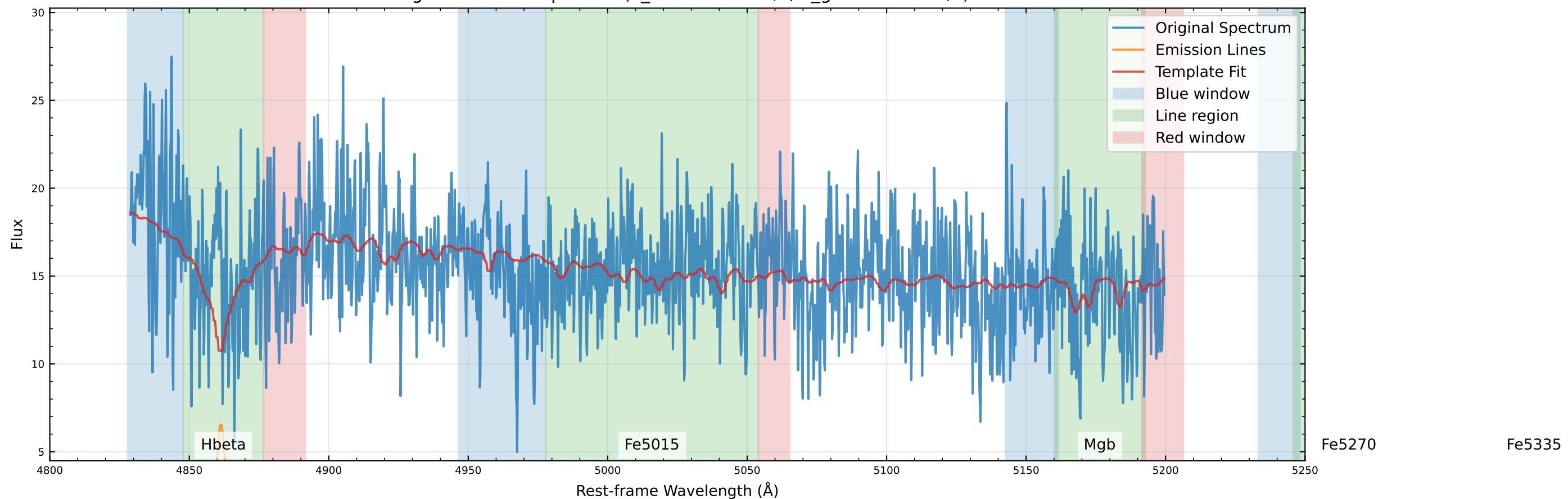
Original Data Comparison (v_star=31.3 km/s, v_gas=-59.4 km/s)
