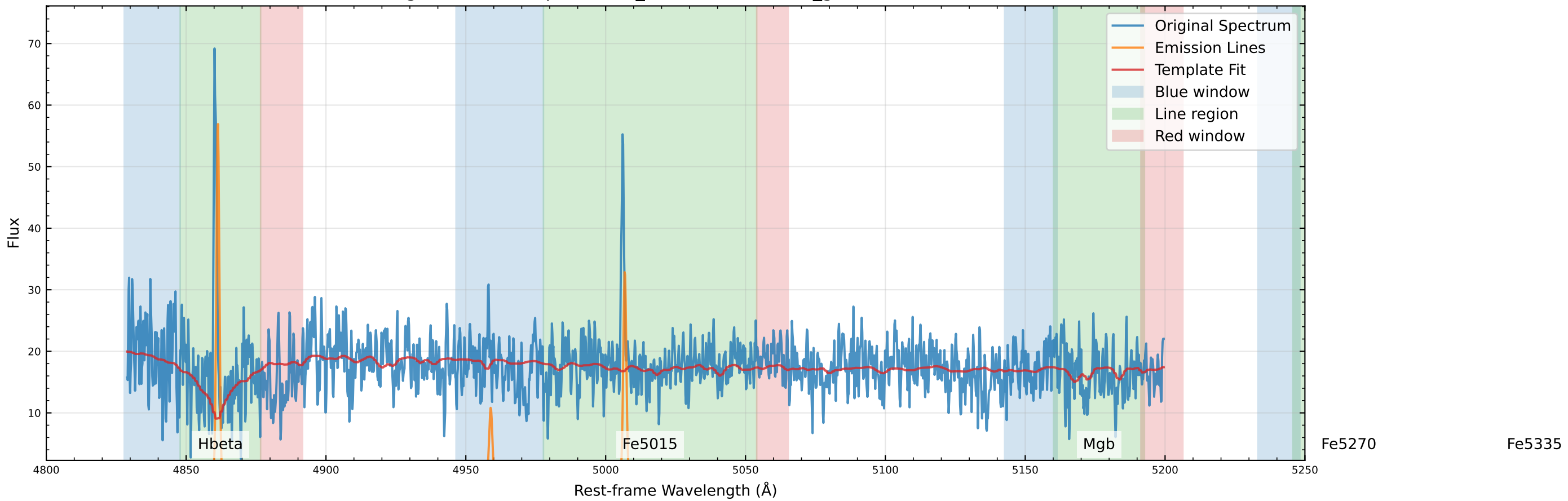
Original Data Comparison (v_star=-48.9 km/s, v_gas=-53.8 km/s)
