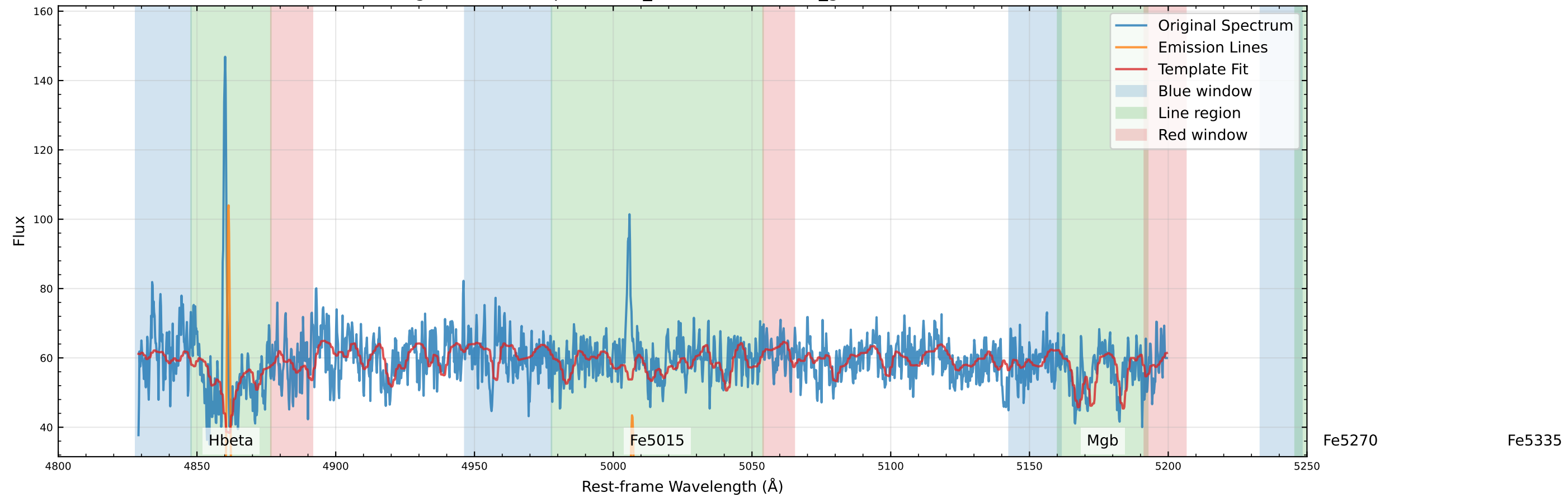
Original Data Comparison (v_star=-81.9 km/s, v_gas=-77.0 km/s)
