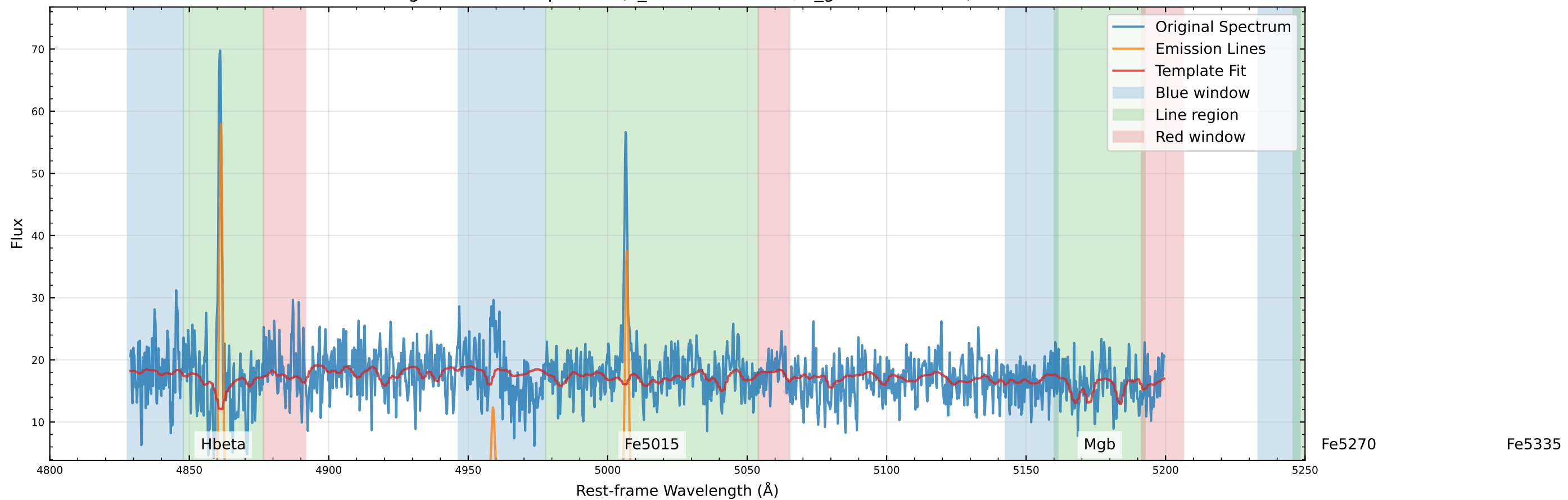
Original Data Comparison (v_star=-16.4 km/s, v_gas=-21.4 km/s)
