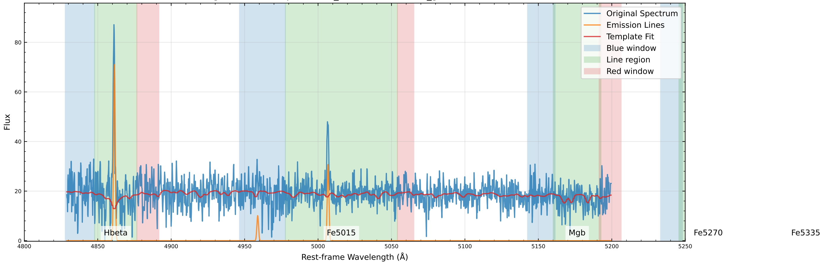
Original Data Comparison (v_star=-50.8 km/s, v_gas=-20.9 km/s)
