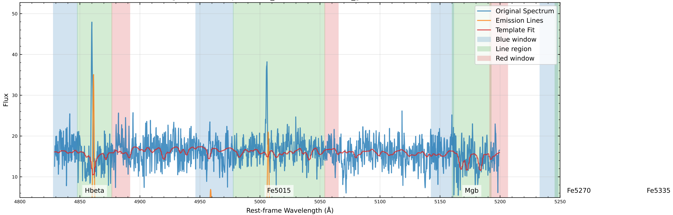
Original Data Comparison (v_star=-106.8 km/s, v_gas=-80.0 km/s)
