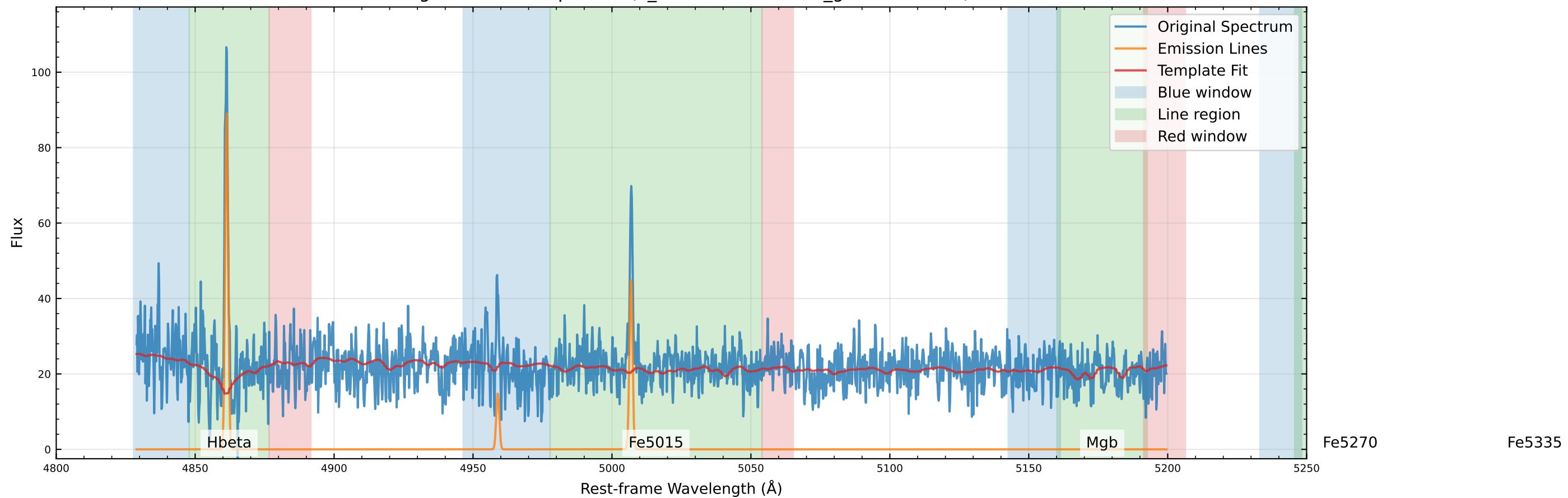
Original Data Comparison (v_star=-28.3 km/s, v_gas=-5.3 km/s)
