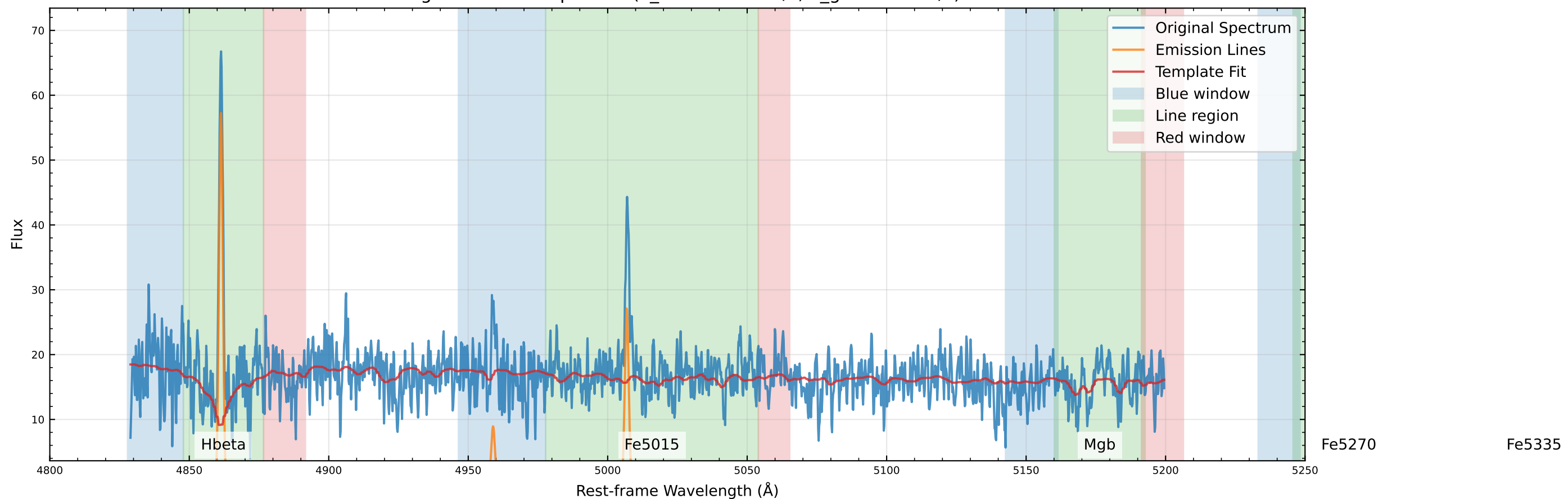
Original Data Comparison (v_star=22.8 km/s, v_gas=4.4 km/s)
