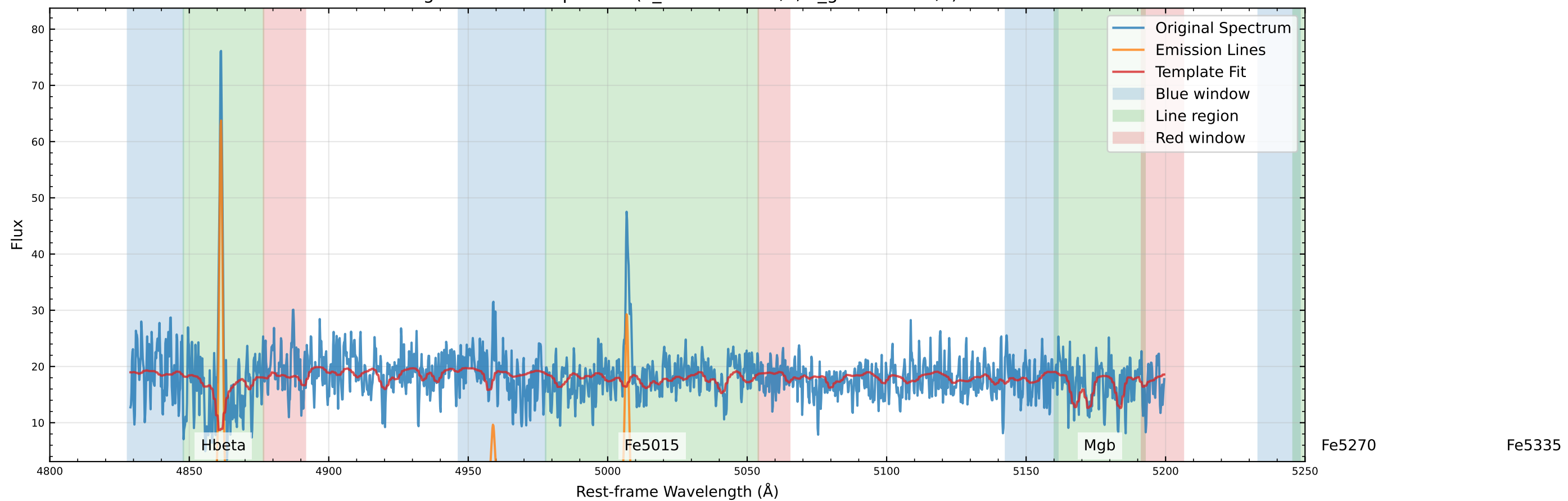
Original Data Comparison (v_star=-9.7 km/s, v_gas=1.3 km/s)
