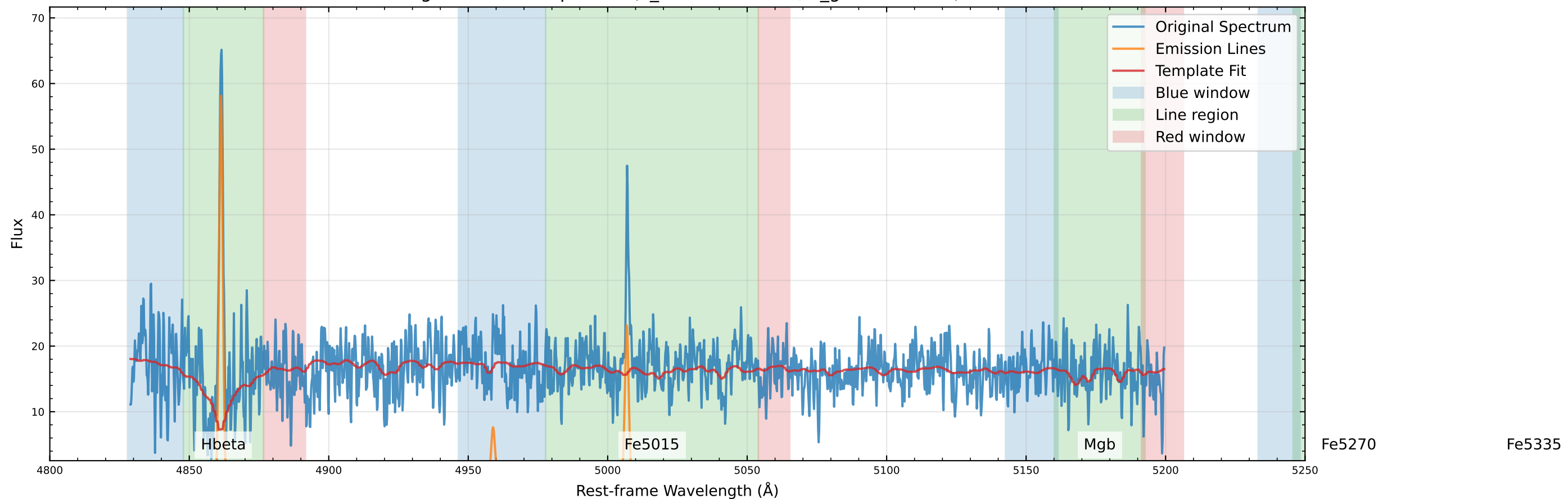
Original Data Comparison (v_star=27.7 km/s, v_gas=7.7 km/s)
