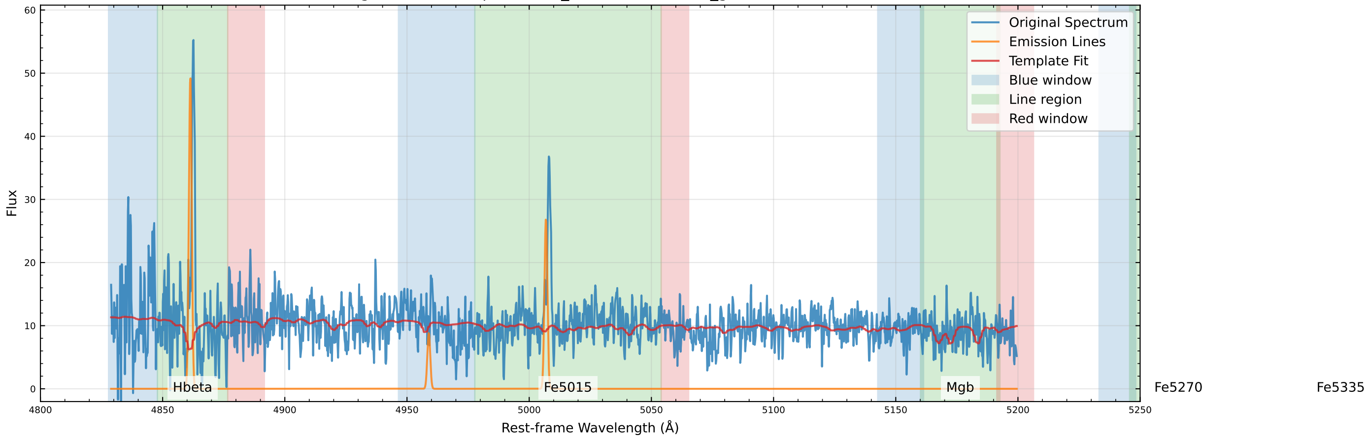
Original Data Comparison (v_star=80.4 km/s, v_gas=74.6 km/s)
