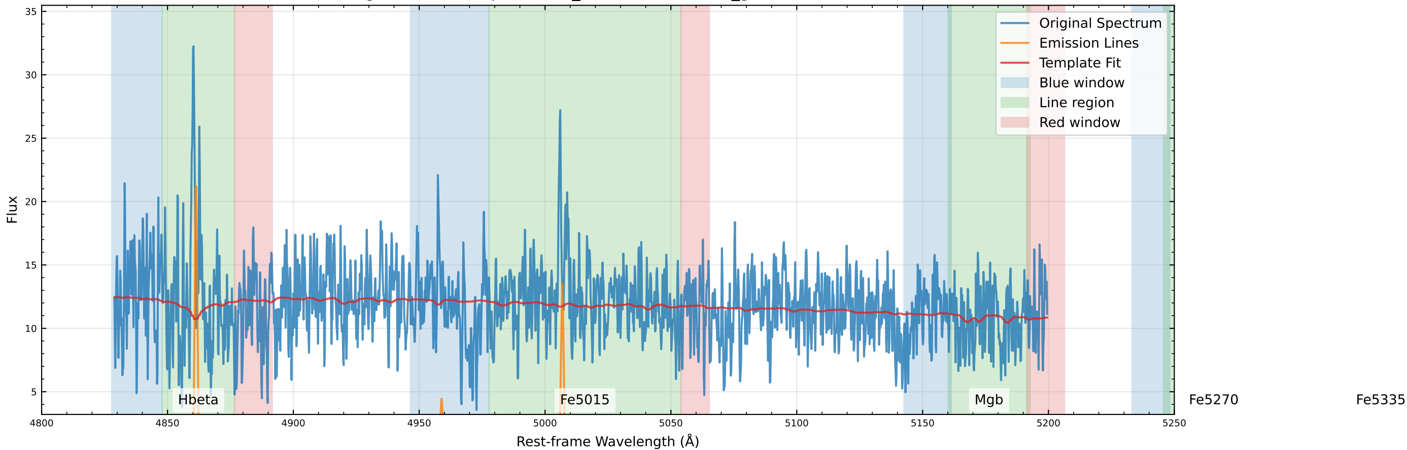
Original Data Comparison (v_star=-12.3 km/s, v_gas=-66.0 km/s)
