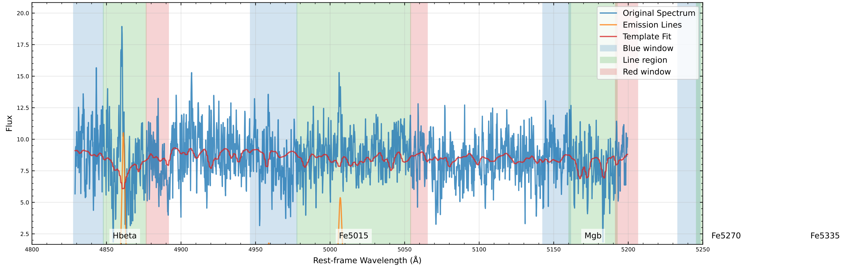
Original Data Comparison (v_star=-43.9 km/s, v_gas=-58.8 km/s)
